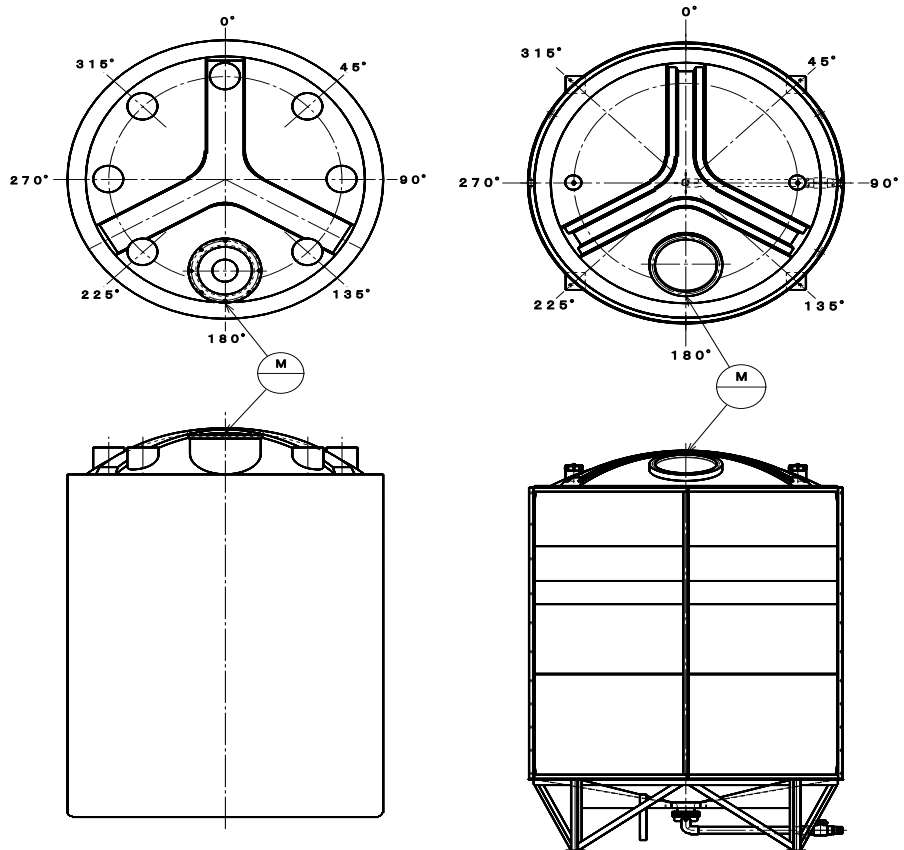
AT-type (No residual liquid tank)
