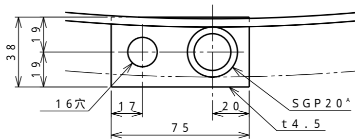
B部詳細 (1:2)
