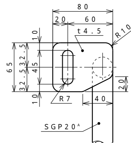
C部詳細 (1:3)
