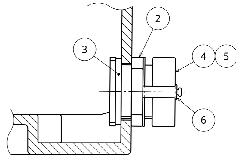
A部詳細 (1:2)
